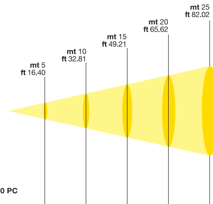
CP70,GX9,5, 1000W
